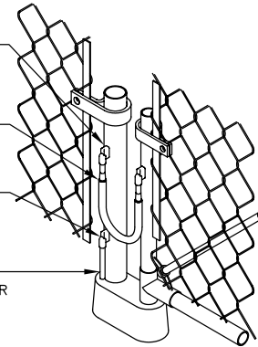
FENCE GROUNDING DETAIL "FG"
