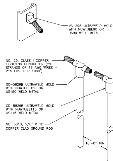
GROUND ROD DETAIL "G"
