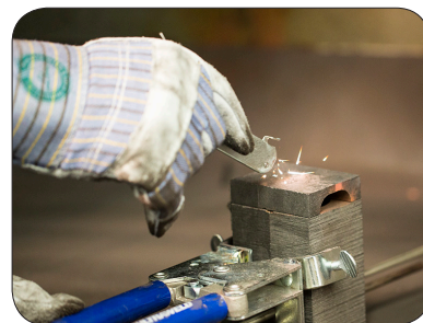
Step 6: Ignite material located on top of the lid using a flint igniter (FLTIG).
